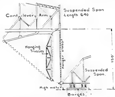
The method of raising the suspended span in position. When the tide came in, the span was afloat and was towed by tugs to the bridge, where it was anchored to the hanging trusses and coupled to the hanger slabs. It was raised by hydraulic jacks
